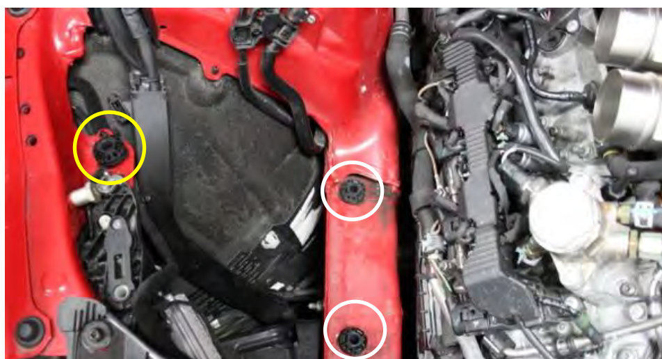
4. Stock Airbox is held in by 3 push mounts circled in the photo. Make sure the Left mount next to the wing is still in place including the rubber – circled in YELLOW.
